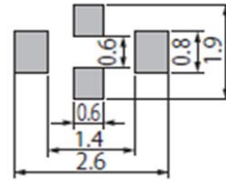
NFM21HC
