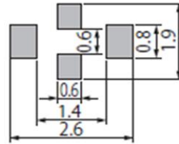
NFM21HC
