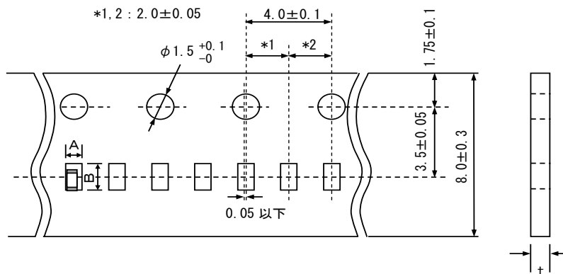
(2) GRM03/GRM15 <紙テ-フ W8P2 包装記号:D/E/J/F>
