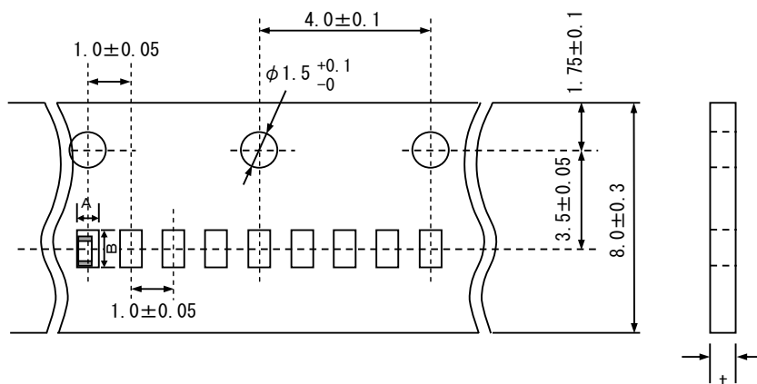
(3) GRM033/GRM155 <紙テ-フ W8P1 包装記号:W>
