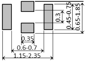
NFM15TC105D NFM15TC435D
