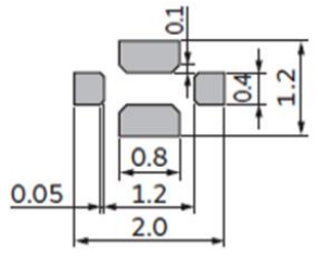
NFM18PS
