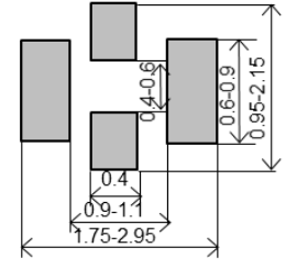
NFM18TC
