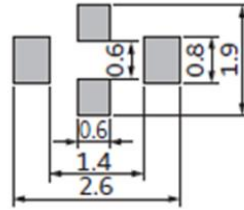
NFM21HC
