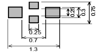
NFM15TC105R
