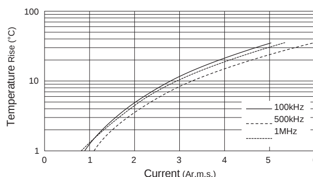
Ripple Current
