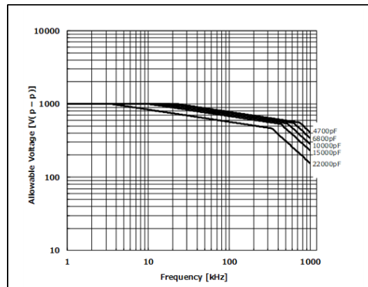
Chip(LxW): 3.2×2.5mm C0G(5C) Char. Rated Voltage : DC1kV
