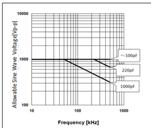
Chip(LxW): 3.2×1.6mm C0G(5C) Char. Rated Voltage:DC1kV
