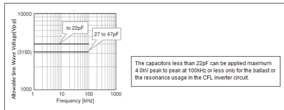
Chip(LxW): 4.5×2.0mm C0G(5C) Char. Rated Voltage:DC3.15kV
