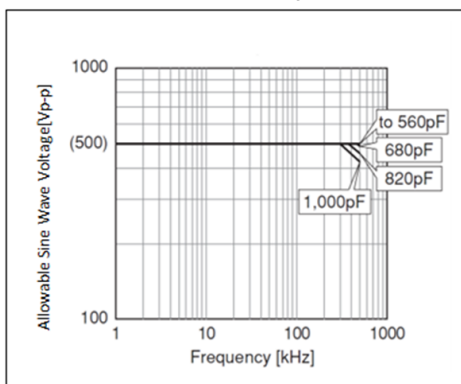
Chip(LxW): 3.2×1.6mm C0G(5C) Char. Rated Voltage:DC500V
