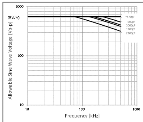
Chip(LxW): 2.0×1.25mm C0G(5C) Char. Rated Voltage:DC630V
