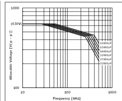
Chip(LxW): 3.2×2.5mm C0G(5C) Char. Rated Voltage:DC630V
