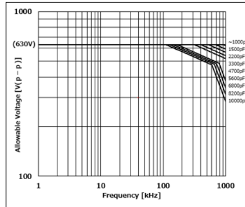
Chip(LxW): 3.2×1.6mm C0G(5C) Char. Rated Voltage:DC630V
