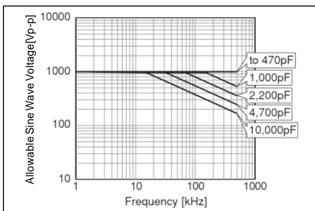
Chip(LxW): 3.2x1.6mm/3.2x2.5mm/4.5x3.2mm/5.7x5.0mm U2J(7U) Char. Rated Voltage : DC1 kV
