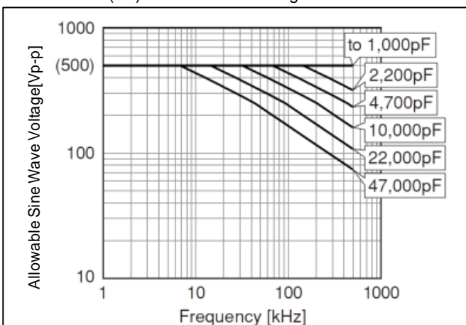
Chip(LxW): 3.2x1.6mm/3.2x2.5mm/4.5x3.2mm/5.7x5.0mm U2J(7U) Char. Rated Voltage : DC500V
