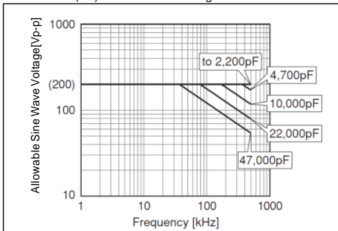
Chip(LxW): 2.0x1.25mm/3.2x1.6mm U2J(7U) Char. Rated Voltage : DC200V
