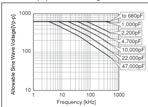
Chip(LxW): 3.2x1.6mm/3.2x2.5mm/4.5x3.2mm/5.7x5.0mm U2J(7U) Char. Rated Voltage : DC630V
