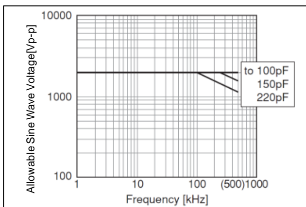
Chip(LxW): 3.2x1.6mm/3.2x2.5mm U2J(7U) Char. Rated Voltage : DC2 kV
