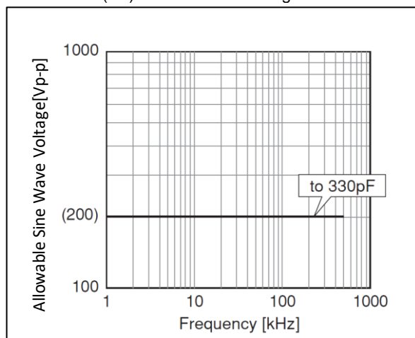
[Frequency VS Allowable Sine Wave Voltage] The surface temperature of the capacitor : 125°C or less (including self-heating)
