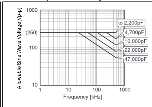
Chip(LxW): 2.0x1.25mm/3.2x1.6mm U2J(7U) Char. Rated Voltage : DC250V
