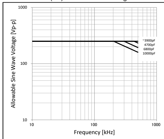
[Frequency VS Allowable Sine Wave Voltage] The surface temperature of the capacitor : 125°C or less (including self-heating)
