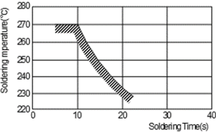
[ Allowable Flow Soldering Temperature and Time ]
