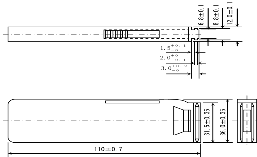
Fig.4 Dimensions of Bulk case
