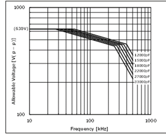
Chip(LxW): 3.2x2.5mm C0G(5C) Char. Rated Voltage:DC630V
