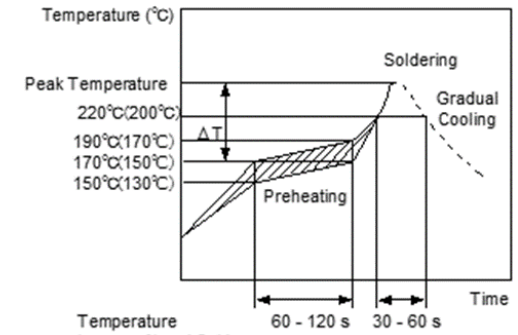
[ Standard Conditions for Reflow Soldering ]
