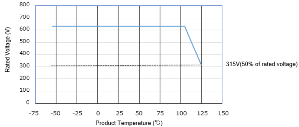
Fig:Derating
