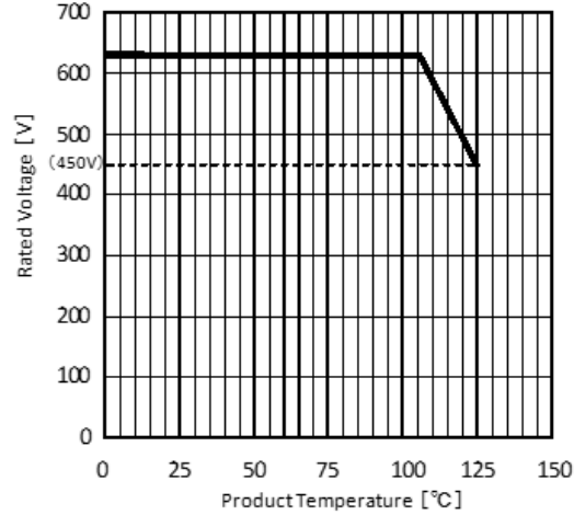
Fig:Derating
