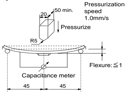
Fig.2 (in mm)
