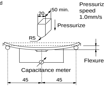
Fig.2 (in mm)
