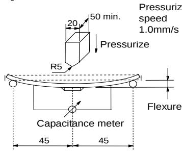
Fig.2 (in mm)
