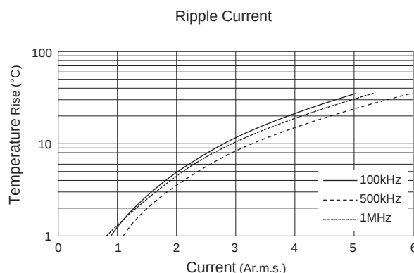
[Example of Temperature Rise (Heat Generation) in Chip Monolithic Ceramic Capacitors in Contrast to Ripple Current] Sample: R(R1) characteristics 10 \mu F, Rated voltage: DC10V
