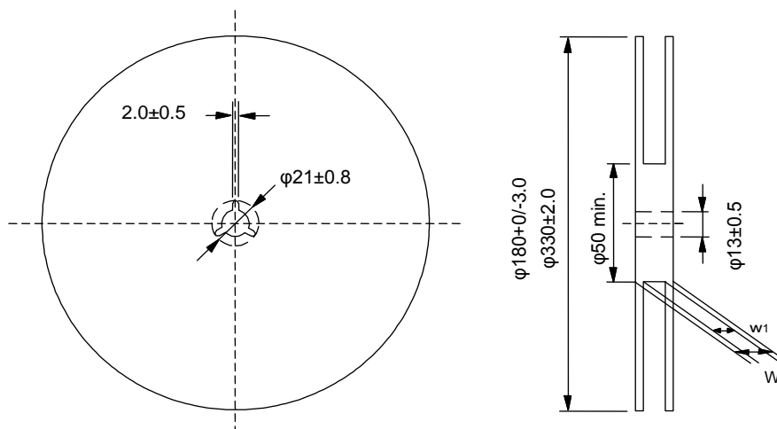
Fig.3 Taping Diagram
