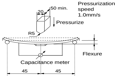
Fig.2 (in mm)
