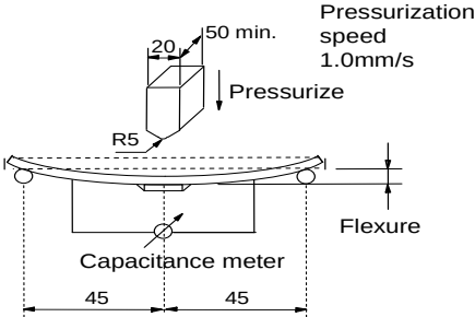
Fig.2 (in mm)
