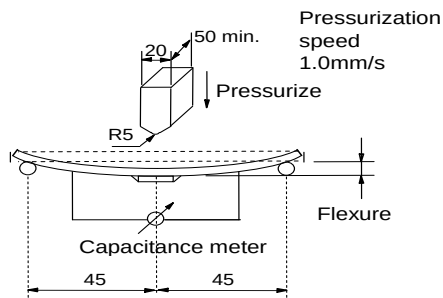
Fig.2 (in mm)
