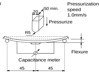
Fig.1 (in mm)
