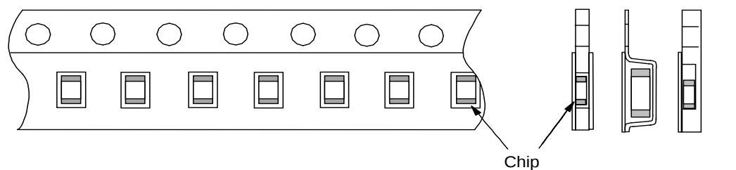
Fig.2 Dimensions of Reel
